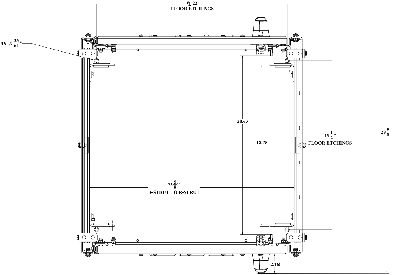
TOP VIEW (NO CEILING OR ALUMASHIELD SHOWN)
