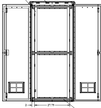
SECTION AD-AD SCALE 1 : 12
