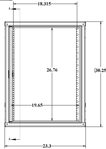
FRONT
