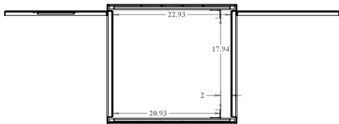
SECTION A-A SCALE 1:8
