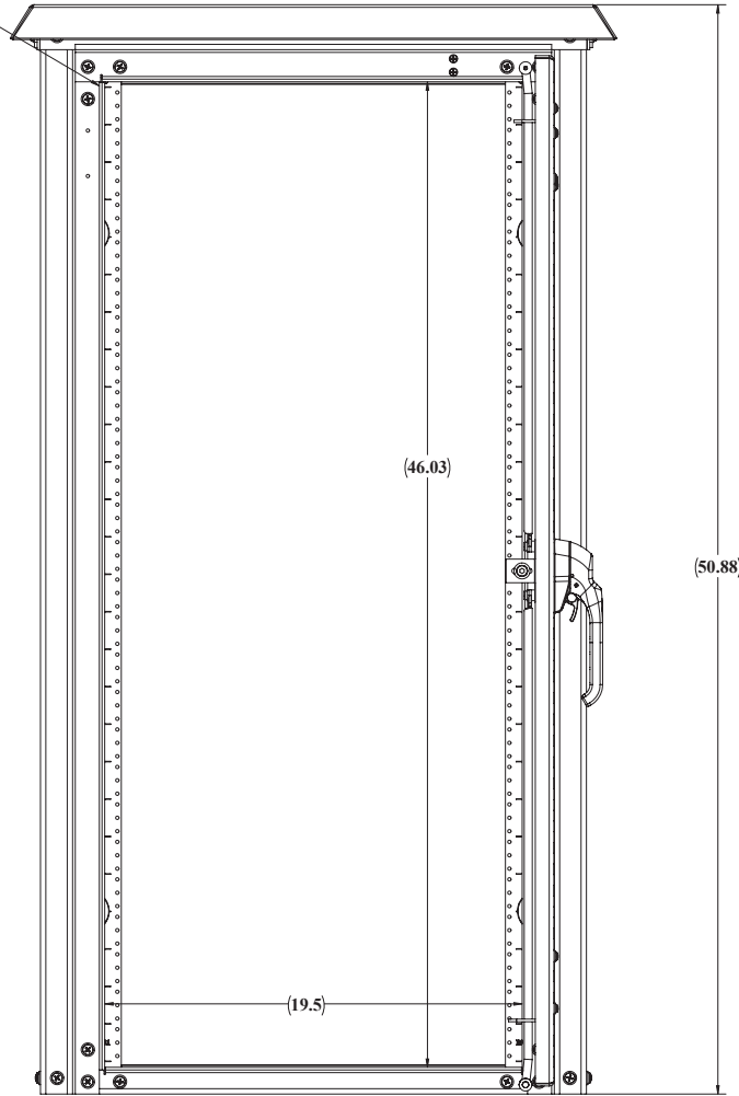
BACK VIEW
