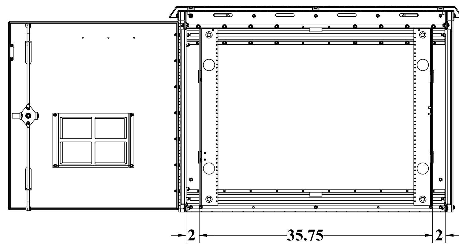
SECTION A-A SCALE 1:9
