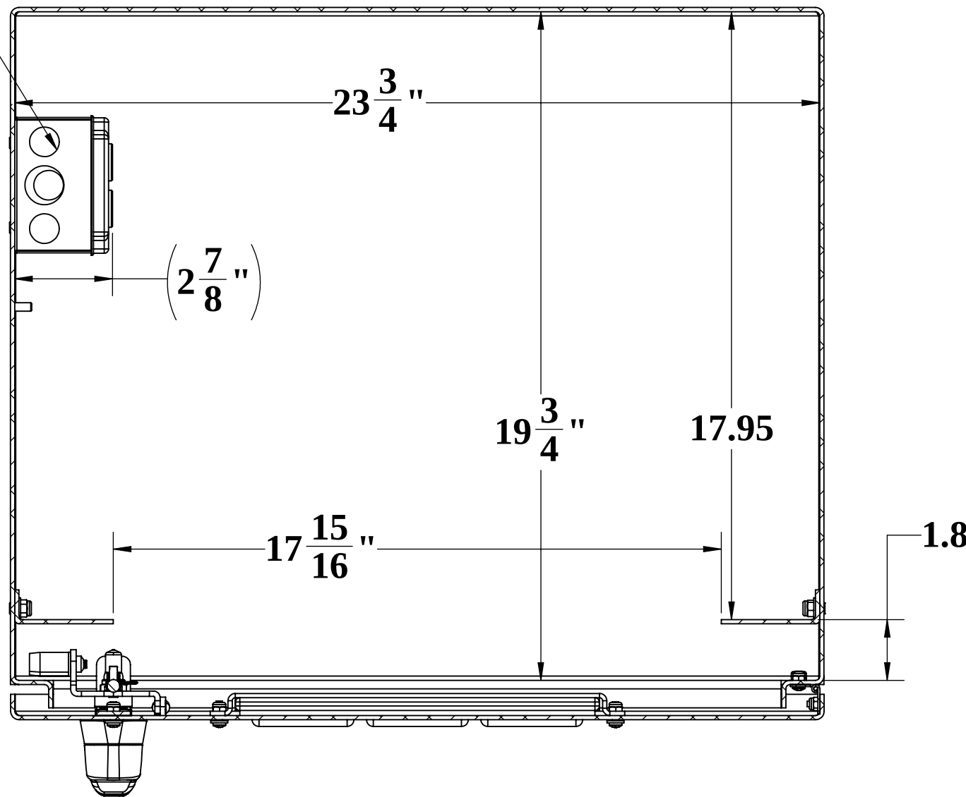
SECTION C-C SCALE 1 : 4
