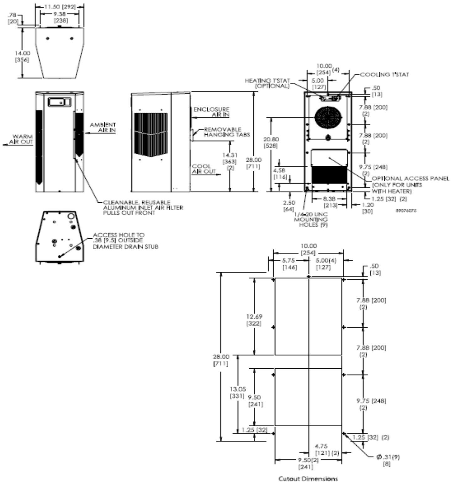
FIGURE 3: nVent /PENTAIR N28 CUT SHEET
